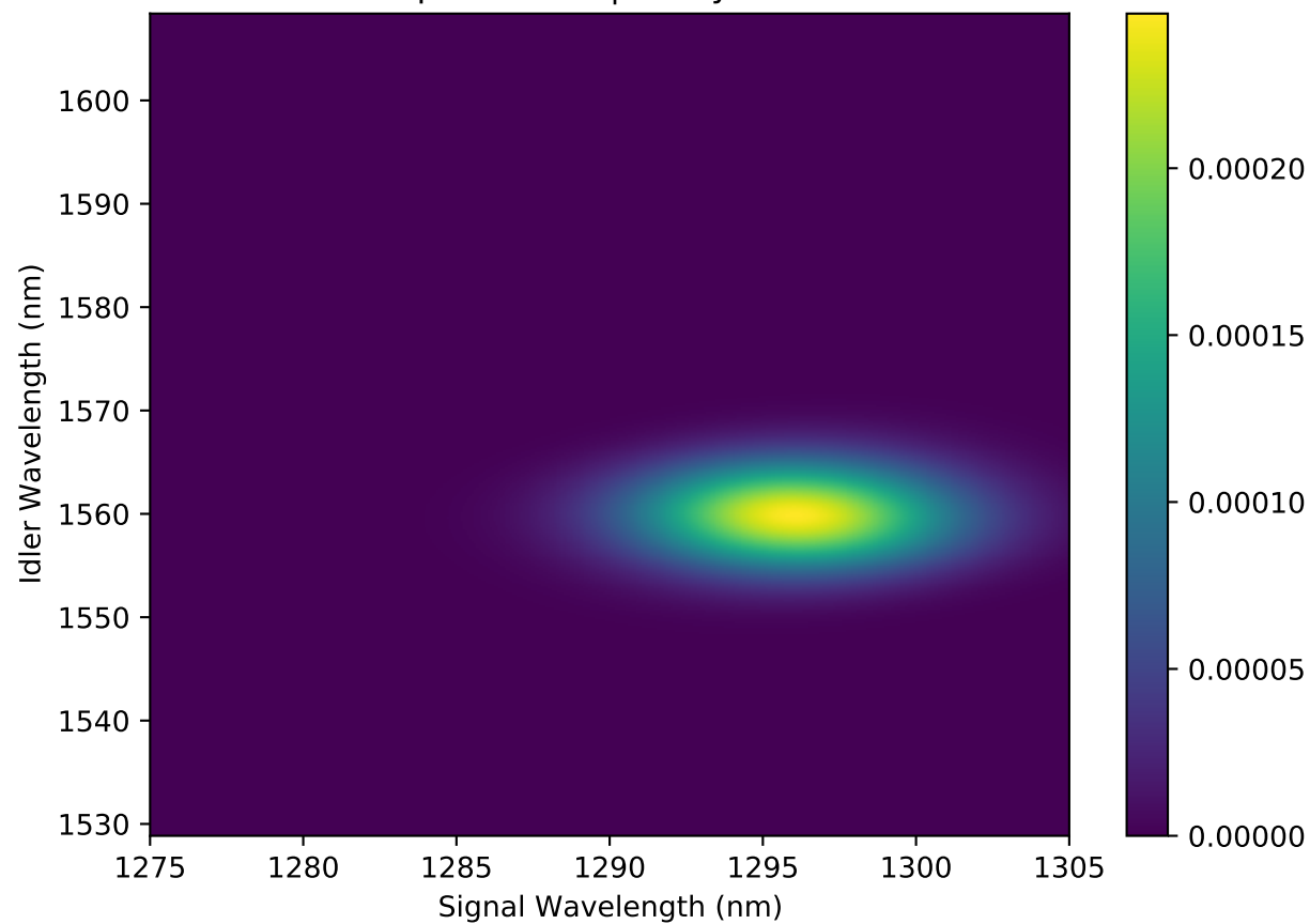
3. Optimized JSA (Theory) Pump=4.40nm | Purity=0.9978
