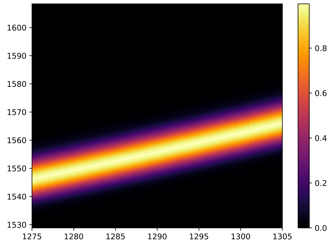
4. Optimized JSA (Exp Reconstruction) Pump=4.40nm | Purity=0.9967
