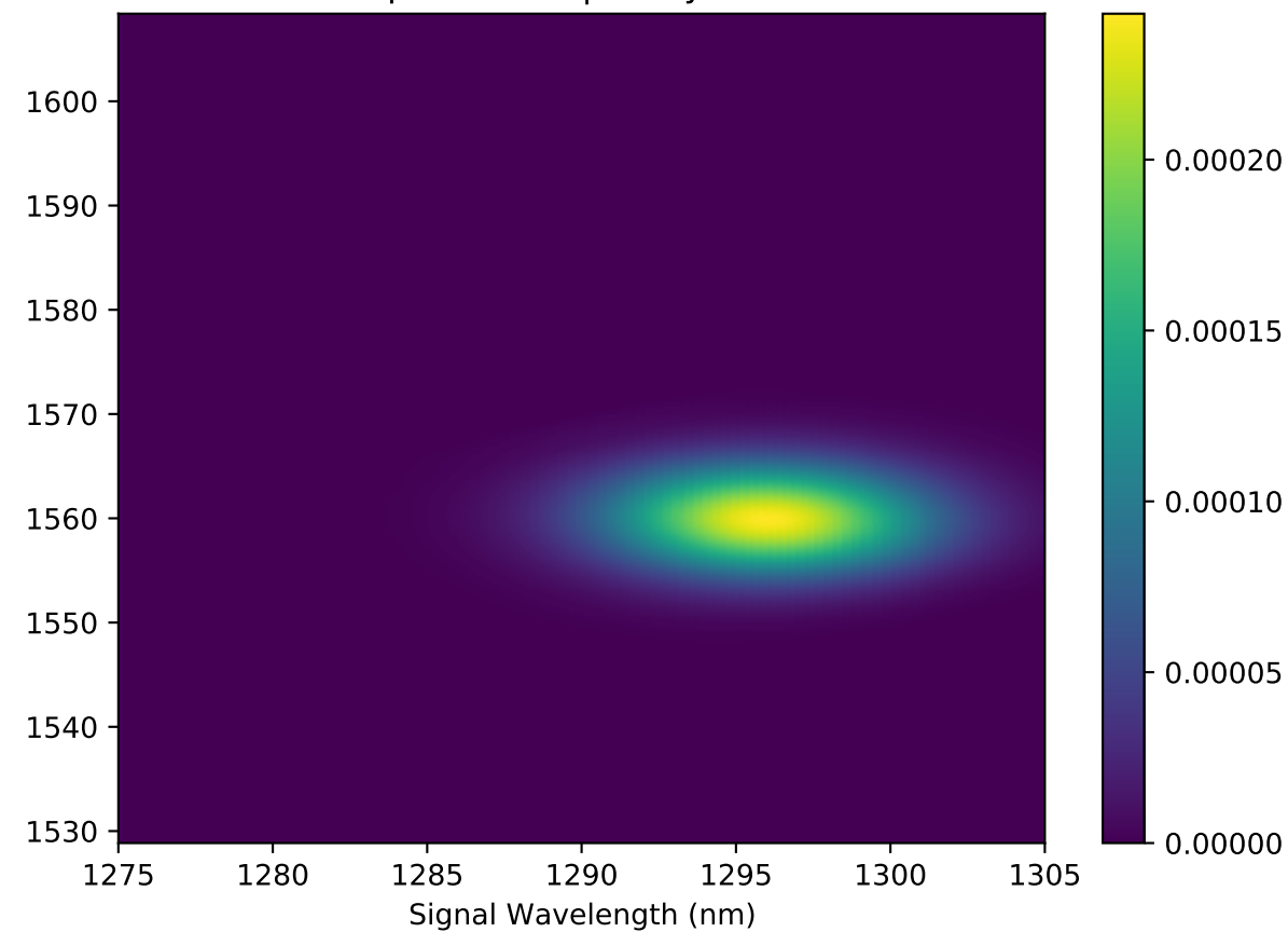
4. Optimized JSA (Exp Reconstruction) Pump=4.40nm | Purity=0.9967
