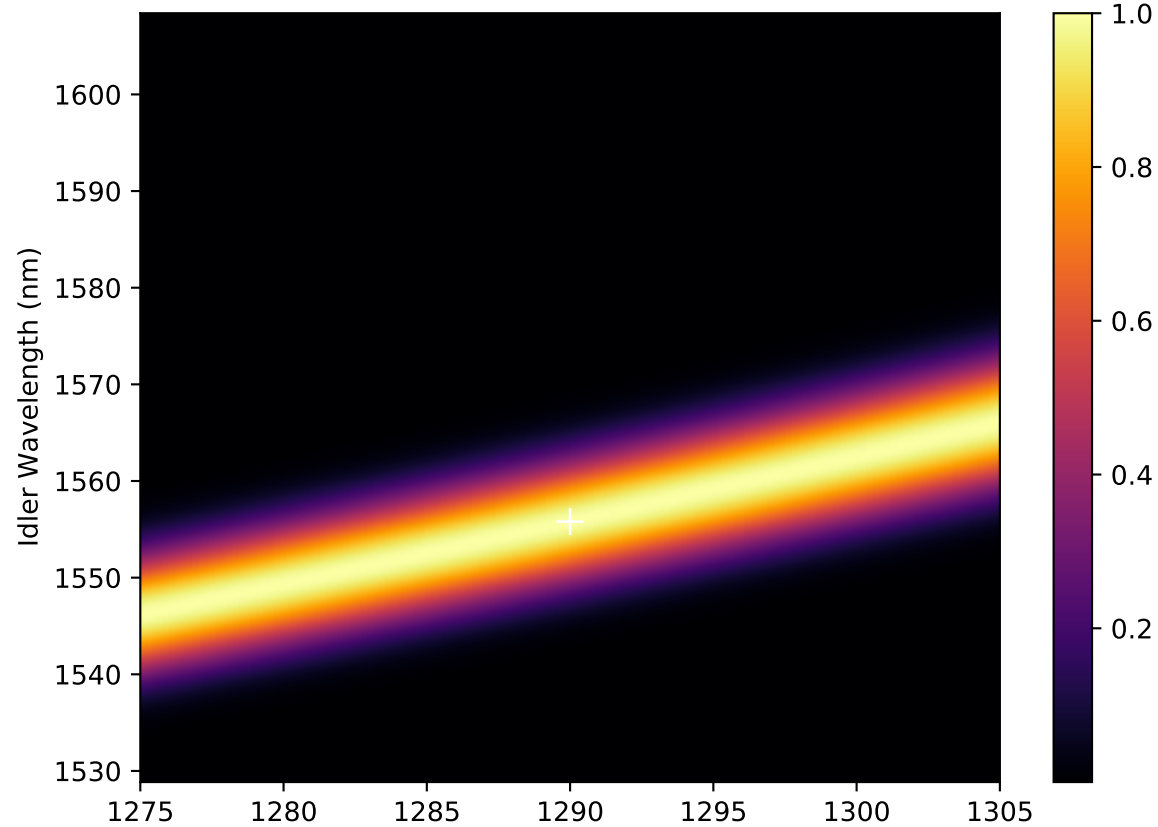
3. Optimized JSA (Theory) Pump=4.40nm | Purity=0.9978
